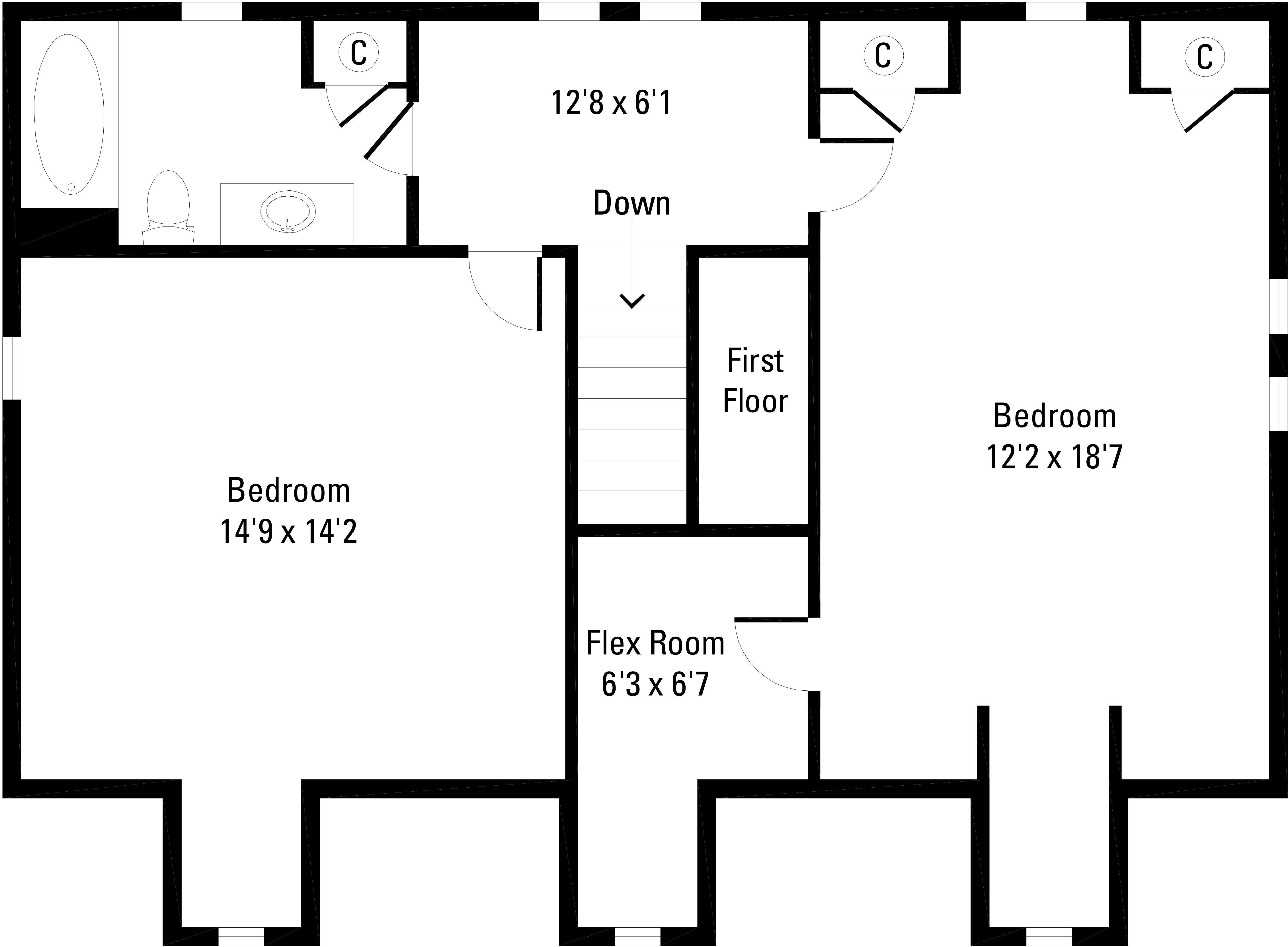
SECOND FLOOR
